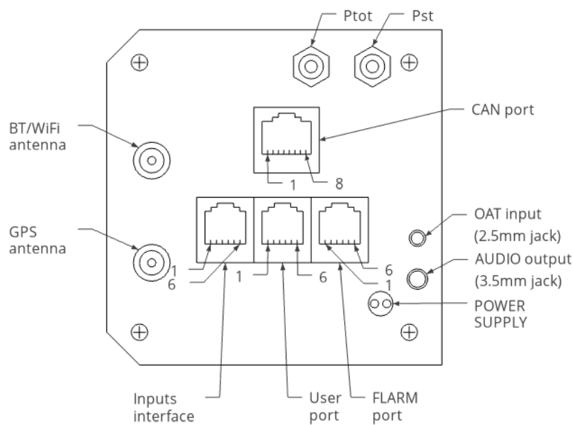
Figure 4. Instrument connections
